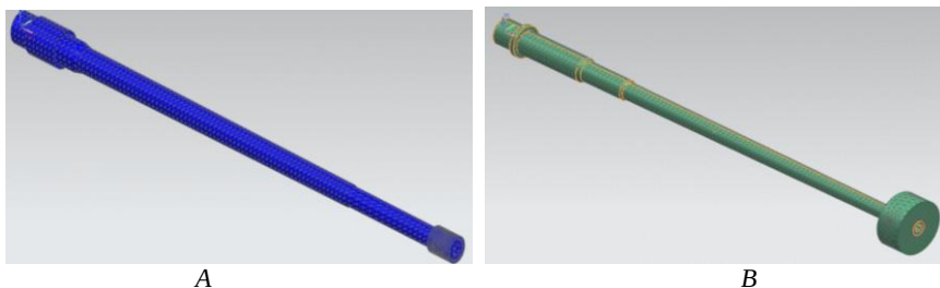
Figure 2. Ballistic barrels three-dimensional model. A- Ballistic barrel that uses cartridges 7,62x39 model 43 year with additionally mounted mass with value 0,025 kg; B- Ballistic barrel that uses cartridges 7,62x54 mm model 1908/30 year with additionally mounted mass with value 0,3 kg.
