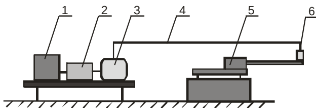
Figure 3. Scheme of experimental investigation devices disposal. 1- computer (program "Lab View 8.5"); 2- DAQ - measurements plate NI USB-6211 – National Instruments; 3- measurements amplifier Type 2635 – Brüel & Kjær; 4- cable; 5- base for ballistic barrel; 6- sensor for vibrations measurement.
