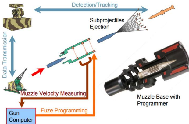
FIG. 2. “SYSTEM INTEGRATION (35MM SKYSHIELD)”
