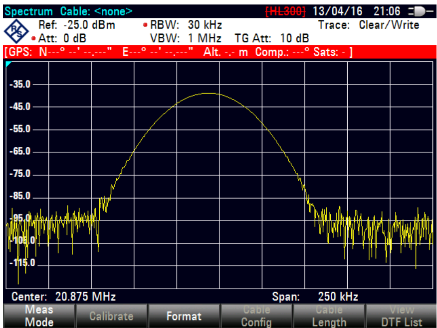
Figure no. 3. 15 m indoor measurment using HF signal
